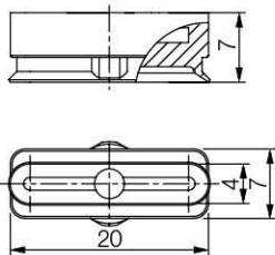
[Rubber part]
